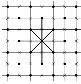
Figure 1: The bonds of 0 in \mathbb{Z}_{\text{ev}}^2
