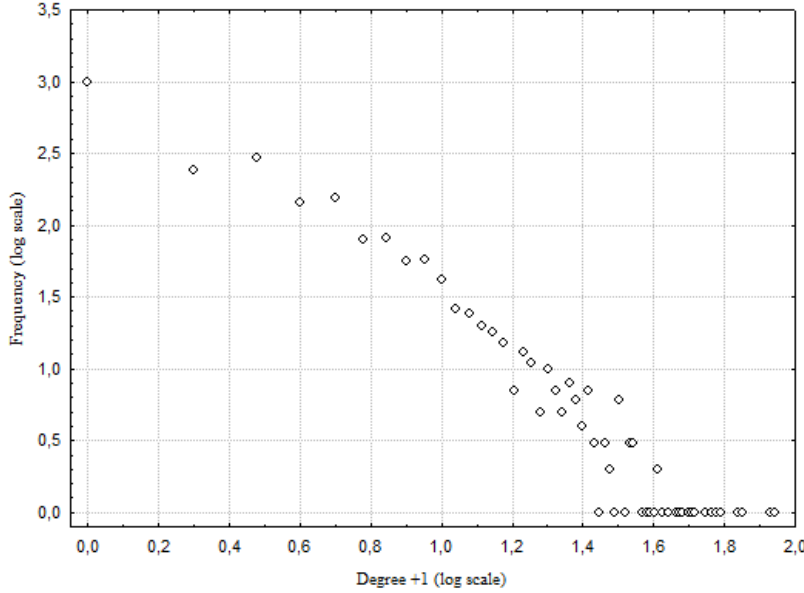
Figure 6 Log-log degree distribution – Brazilian Network
