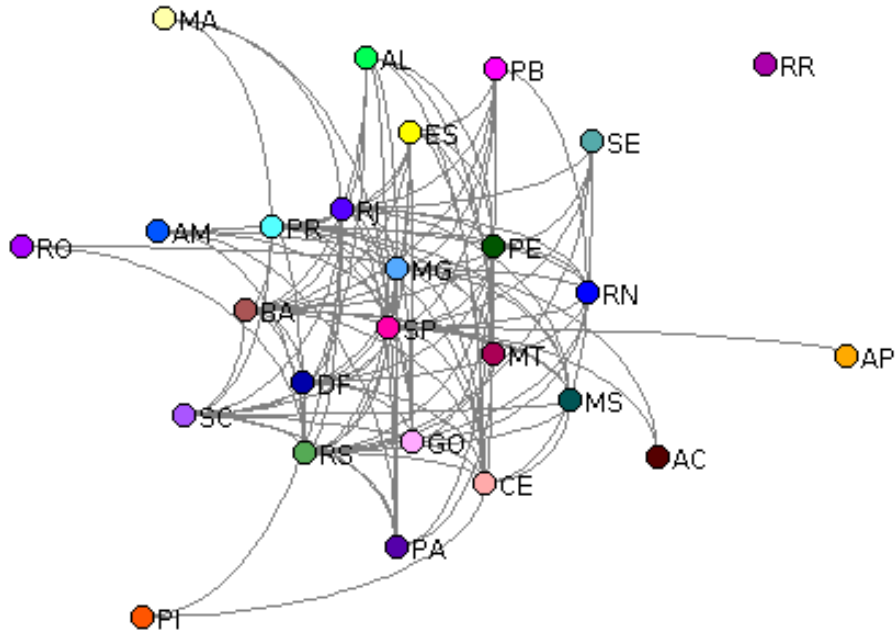
Figure 1 P&S collaboration network – Brazilian states network
