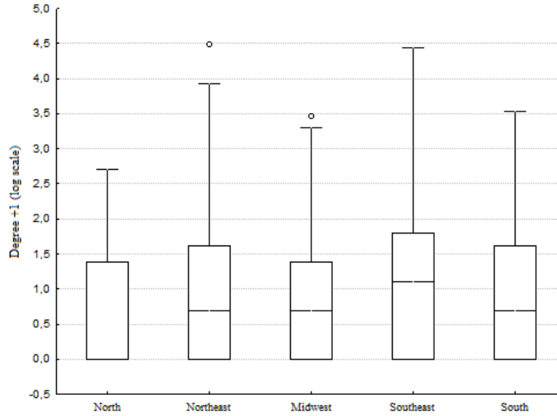
Figure 7 Distribution of \log(\text{degree} + 1) by Brazilian region
