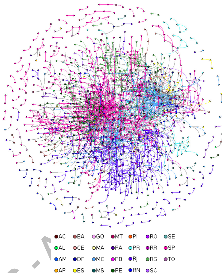
Figure 4 Probability and Statistics Researchers Collaboration Network - reorganized.
