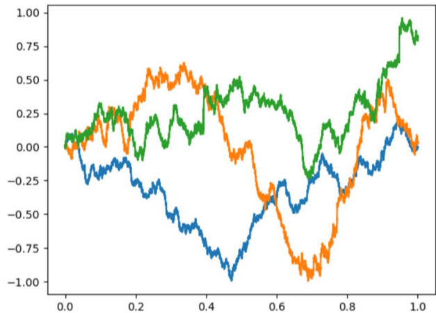
FIG. 3. Sample paths of the fractional Brownian Motion (blue), the Rosenblatt process (orange) and the Hermite process of order 3 (green) with Hurst parameter 0.6.
