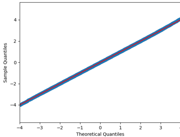
FIG. 9. Qq-plot comparing the empirical quantiles of the set (54) in the case of the fractional Brownian motion ( d = 1 ) to the quantiles of the cumulative distribution function of a \mathcal{N}(0, 1) Gaussian random variable.
